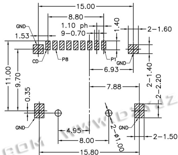
PCB LAYOUT TOP VIEW (TOLERANCE: ±0.05)
